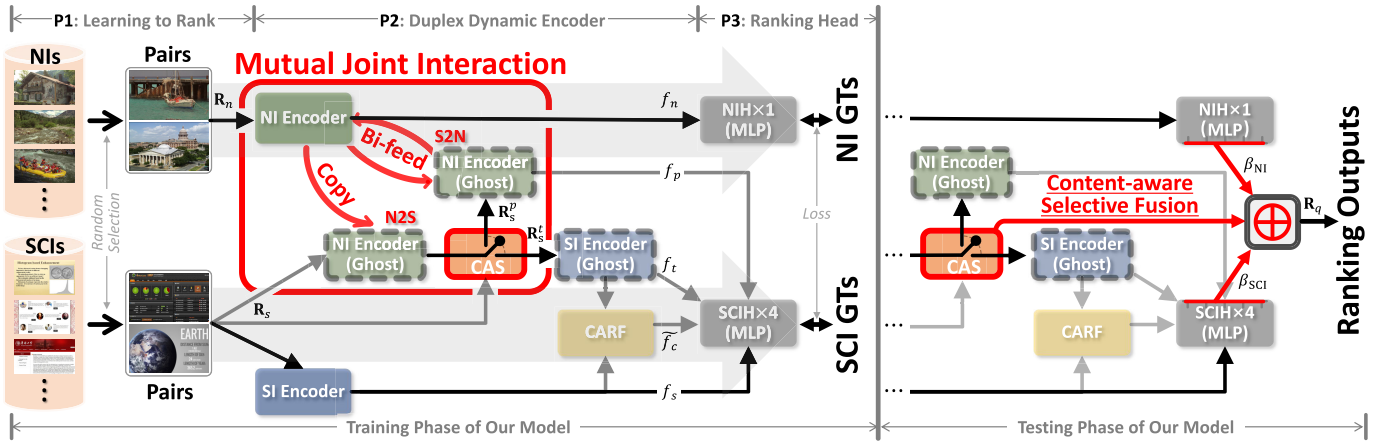
Fig. 3. The pipeline of our approach mainly consists of three major parts. In the training phase, after pre-processing the datasets by learn-to-rank strategy (P1), we first feed the paired images to the NI stream (the upper light grey arrow) and the SCI stream (the lower light grey arrow) of the duplex dynamic encoder (P2), then obtain two relative ranking scores (P3). Specifically, the “content-aware” data switch (CAS) aims at letting the model automatically enhance the commonness and compress the discrepancies between the two tasks. The term “Bi-feed” refers to the shared architectures and parameters between NI Encoder and NI Encoder (Ghost), i.e. , S2N, and the mutual weight updates. In contrast, “Copy” signifies unidirectional weight transfer from NI Encoder to NI Encoder (Ghost), i.e. , N2S. During the testing phase, we employ content-aware selective fusion to generate the final relative ranking score. The symbol “ \oplus ” indicates the weighted addition of the two scores.
