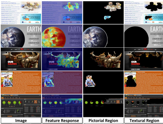
Fig. 6. Visualization of pictorial and textural regions in the SCIs generated by the “content-aware” data switch.
