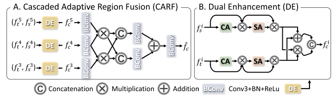
Fig. 4. Detailed architecture of CARF. CA: Channel Attention, SA: Spatial Attention. All upsampling and downsampling are omitted.
