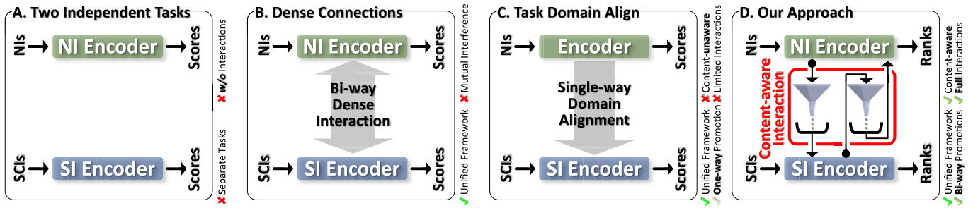
Fig. 2. Most existing methods treated NI-IQA and SCI-IQA as independent tasks (A). However, the most intuitive multi-task methodology could lead the two tasks to interfere (B). Also, the most recent domain alignment-based method [6] (C) only enables single-way interaction with limited performance gain. The key highlight of our approach (D) is the proposed content-aware interaction, which enables the two tasks to interact fully while avoiding “domain shifts” and “dataset misalignment”-induced side effects. We use ✓ and ✗ to denote advantages and disadvantages between our proposed method and the existing methods.
